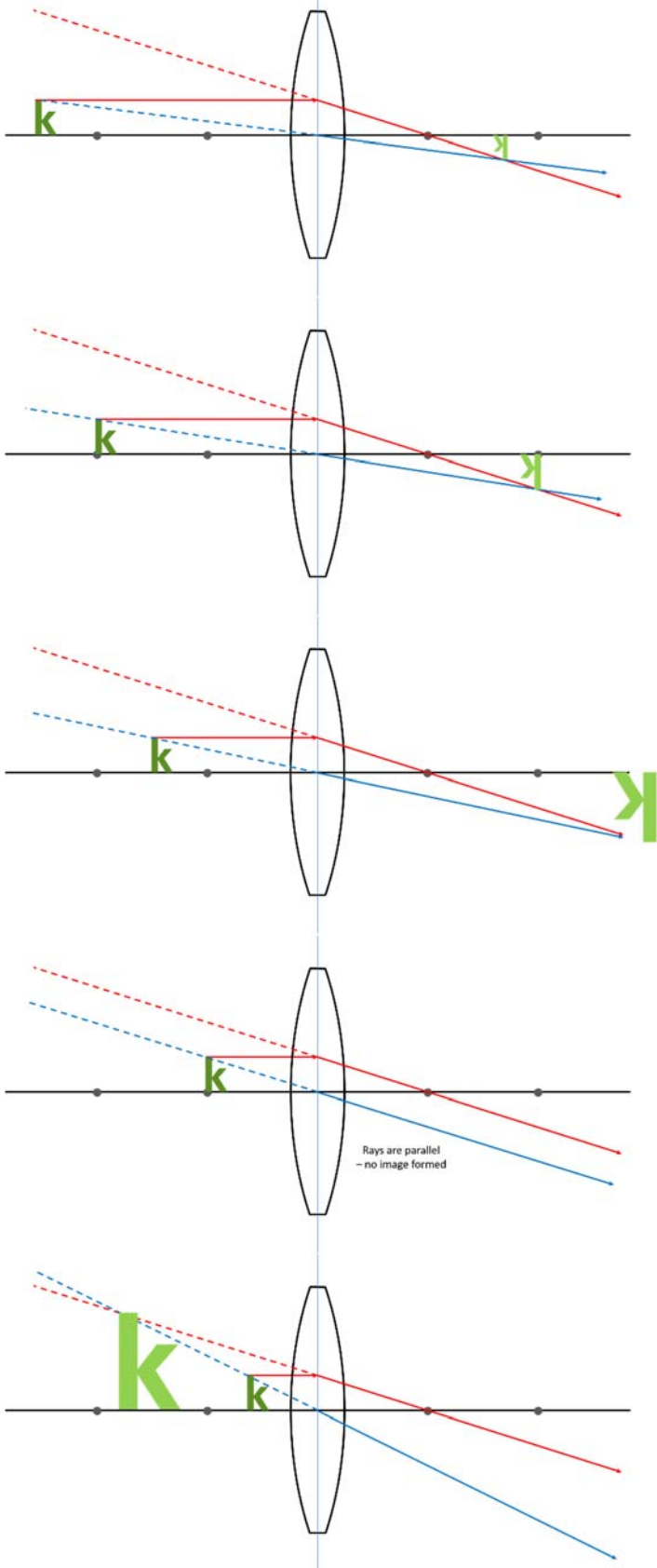
Convex Lens
